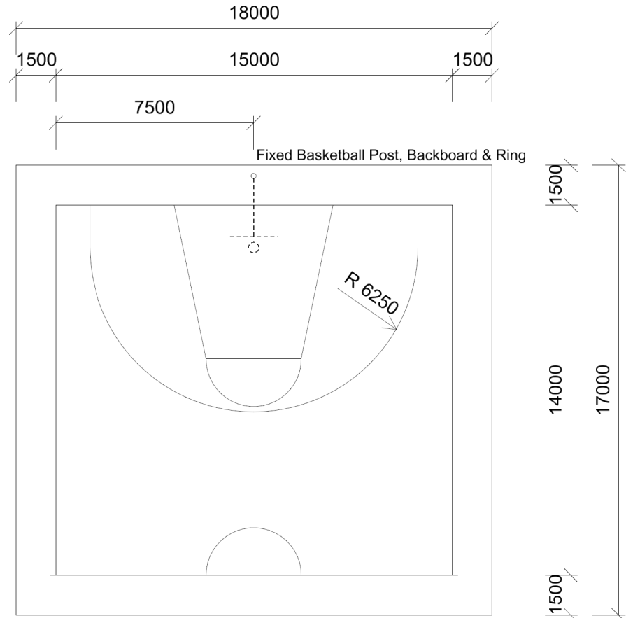
289 sq.m Basketball (Half Court) - 50mm Yellow lines Dimensions to inside of lines
