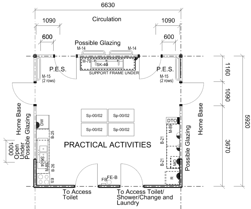
Floor Area shown 39.25 sq.m (includes 6 sq.m P.E.S.)
