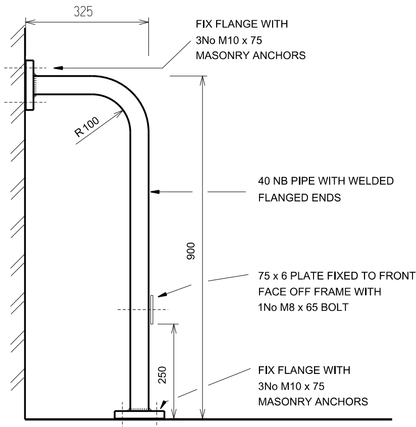
SIDE ELEVATION - SEPARATING FRAMES
