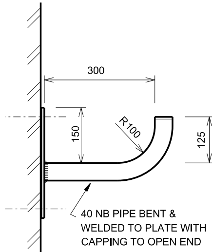
SIDE ELEVATION - HOSE HOOK
