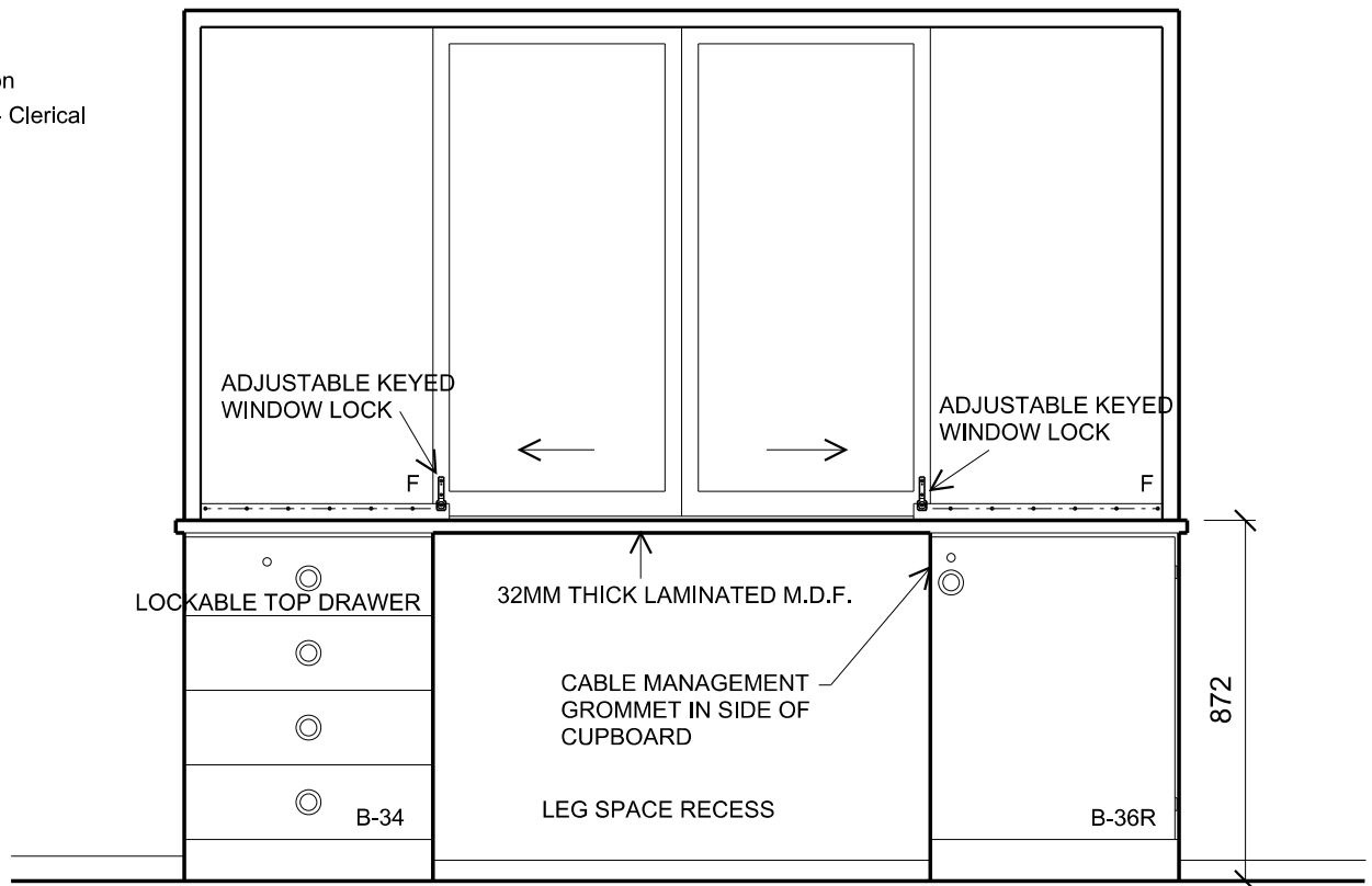
ADMINISTRATION - CLERICAL - ELEVATION
