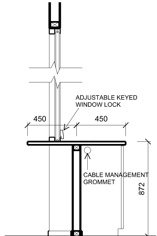
SECTION THROUGH WINDOW OPENING NTS
