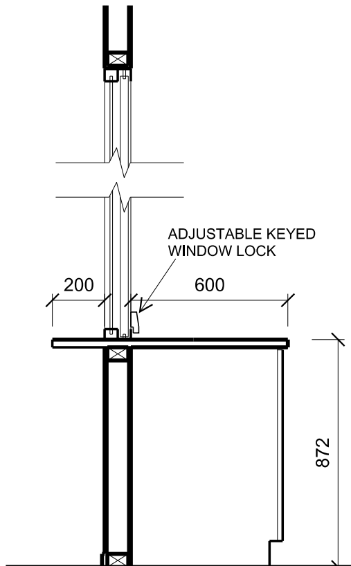
SECTION THROUGH CUPBOARD
