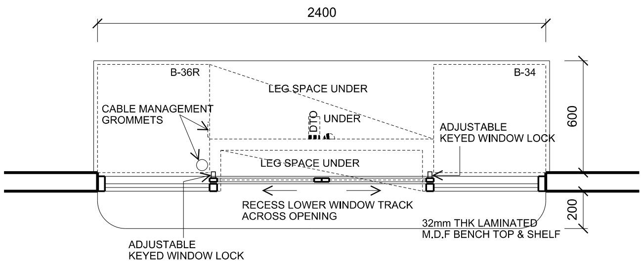
ADMINISTRATION - CLERICAL - PLAN
