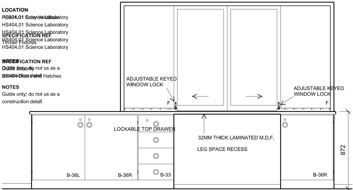
CLERICAL/DUPLICATING - ELEVATION
