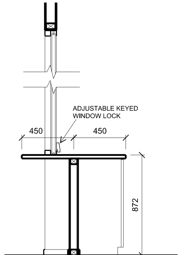
SECTION THROUGH WINDOW OPENING NTS
