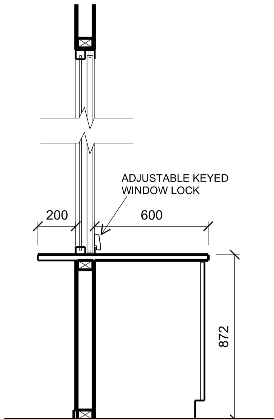
SECTION THROUGH CUPBOARD
