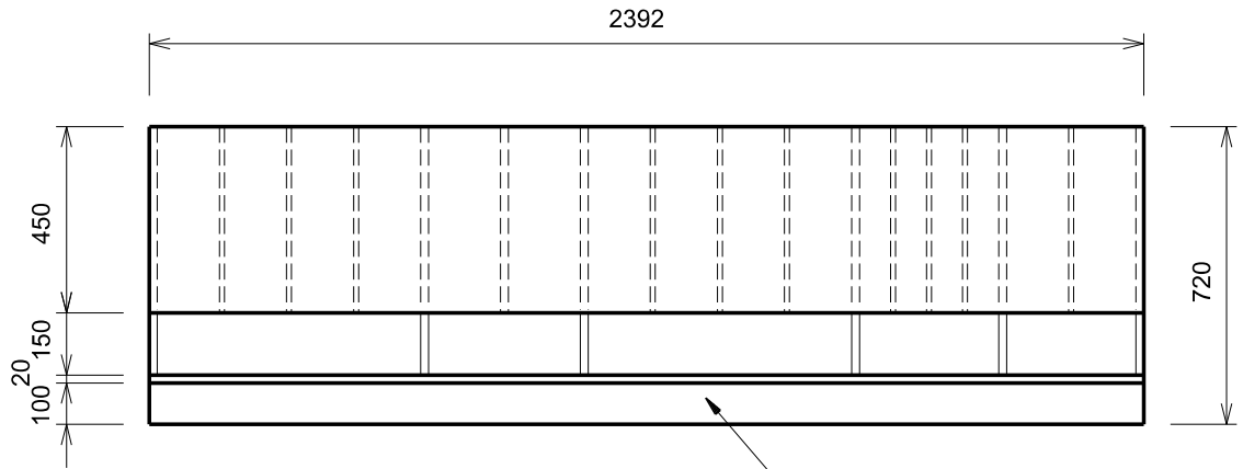
ELEVATION - BAT RACK
