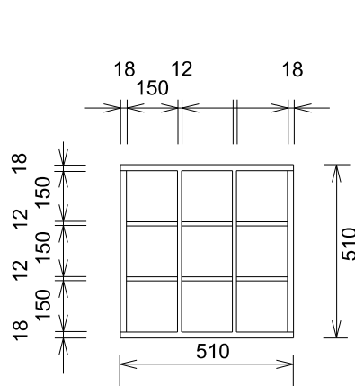
PLAN - BAT RACK
