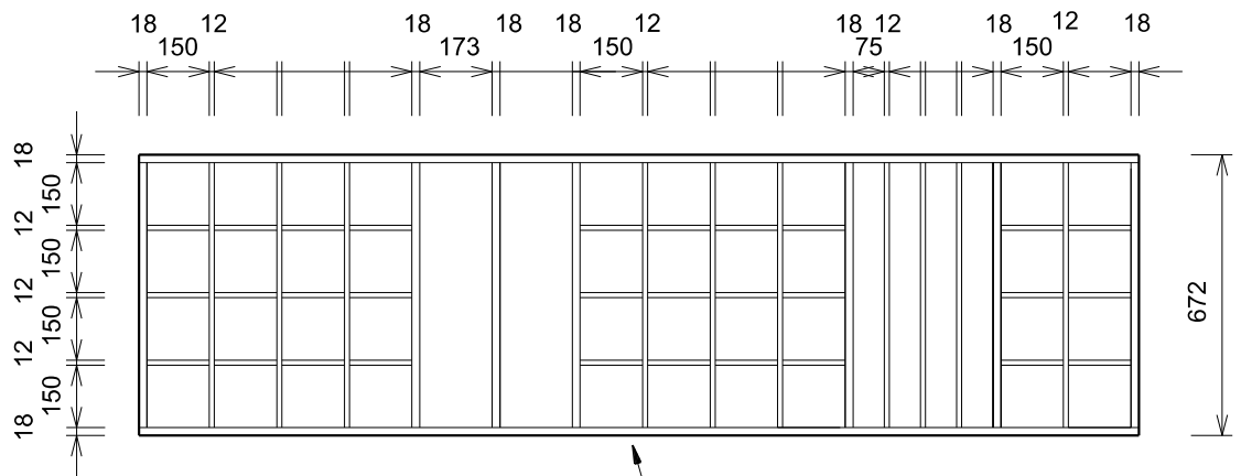
PLAN - BAT RACK
