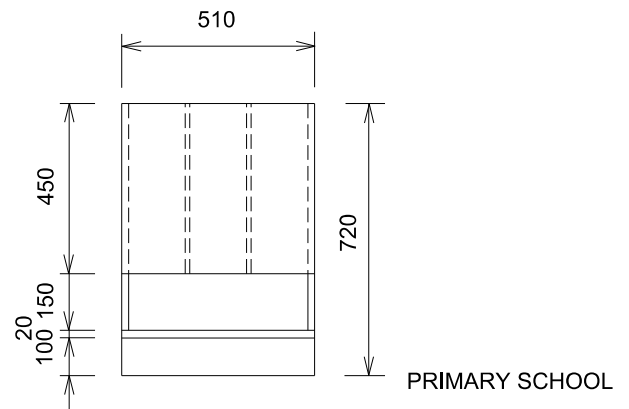
ELEVATION - BAT RACK
