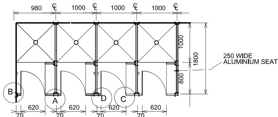
PLAN - SHOWERS
