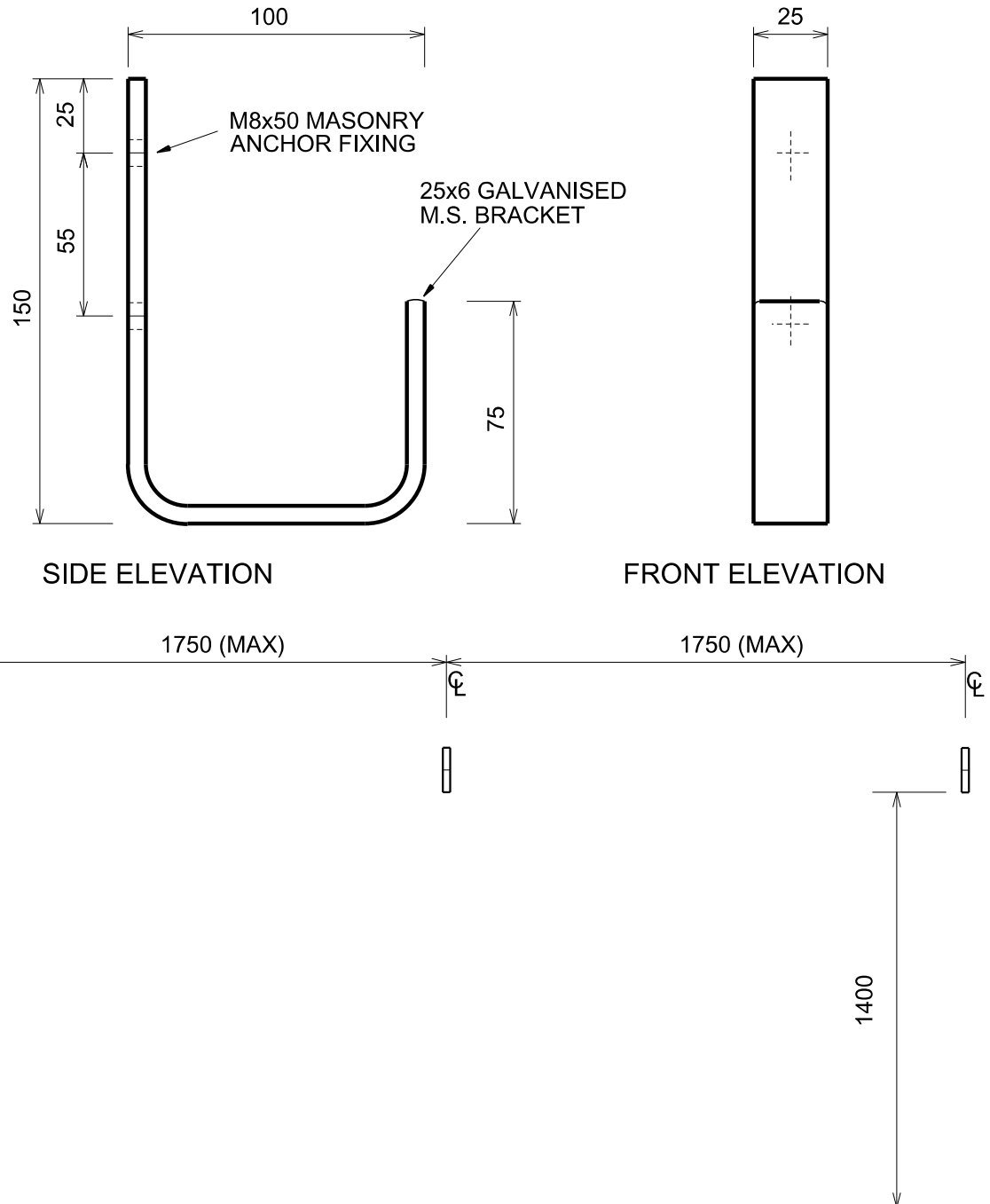
ELEVATION - HIGH JUMP RACKS
